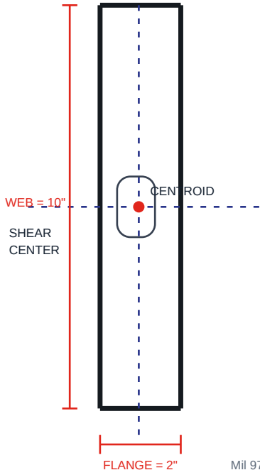
CAD SECTION
