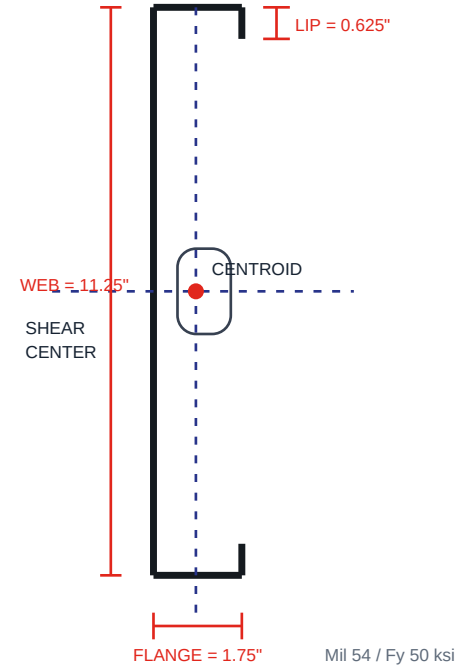
CAD SECTION
