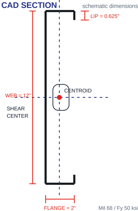
CAD SECTION
