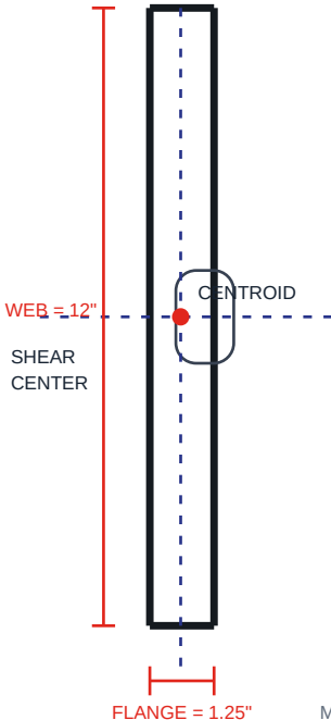
CAD SECTION
