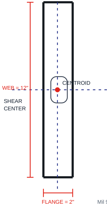
CAD SECTION
