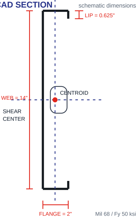
CAD SECTION
