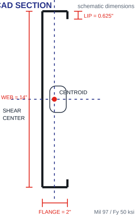
CAD SECTION
