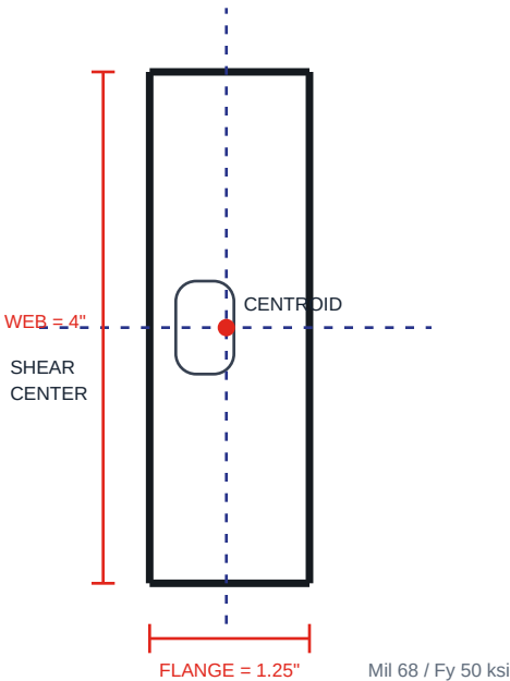
CAD SECTION
