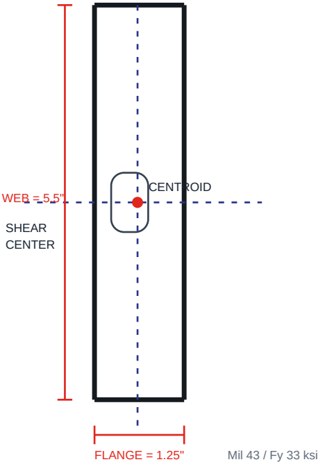
CAD SECTION
