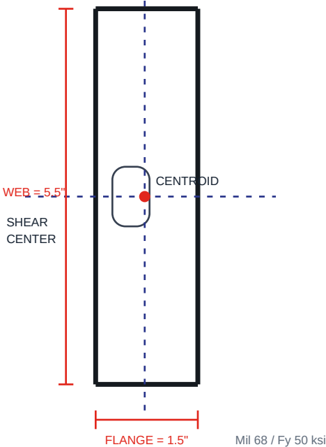
CAD SECTION
