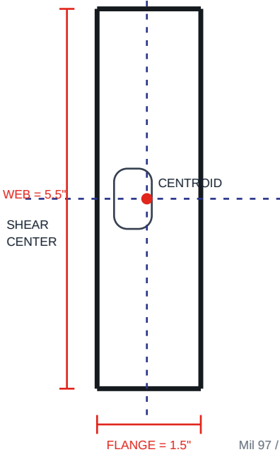
CAD SECTION
