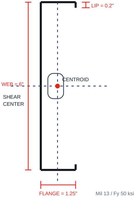
CAD SECTION
