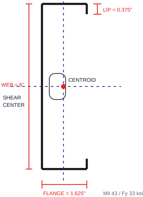
CAD SECTION
