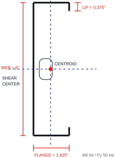
CAD SECTION
