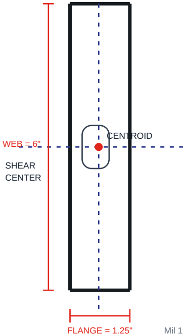
CAD SECTION
