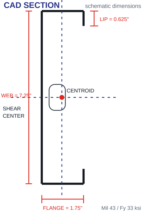
CAD SECTION
