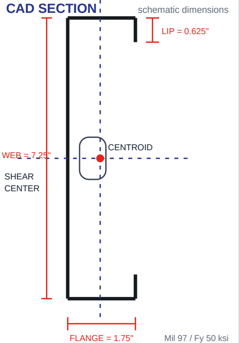
CAD SECTION
