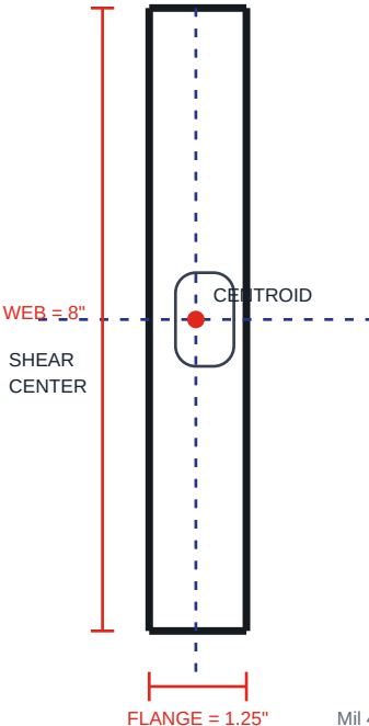
CAD SECTION
