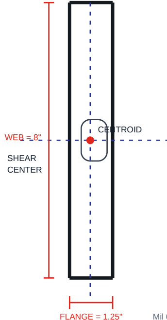
CAD SECTION
