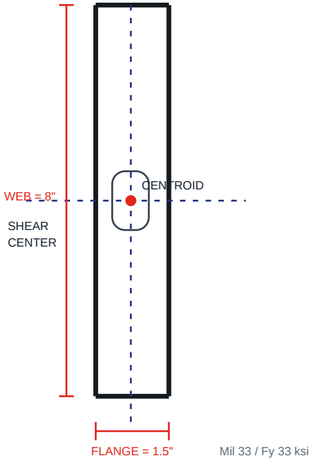
CAD SECTION
