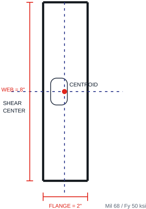
CAD SECTION
