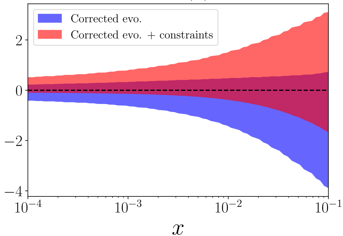
x\Delta G(x)
