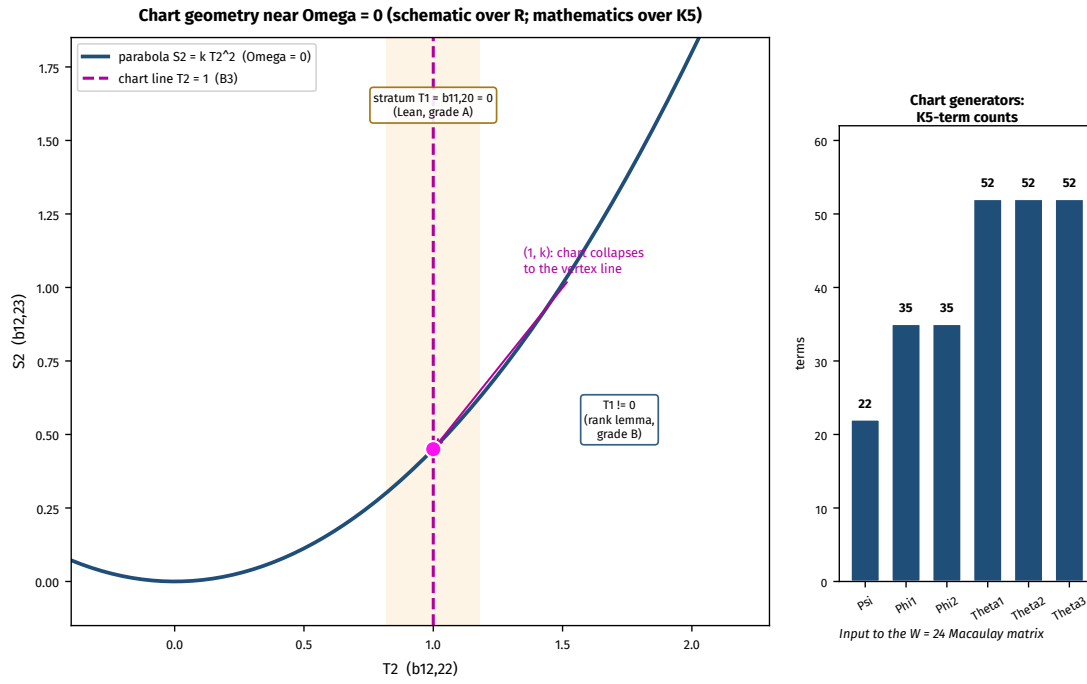
Figure 3: Chart geometry near \Omega = 0 . Main panel: the (T_2, S_2) -plane drawn schematically over \mathbb{R} for illustration (the mathematics is over K_5 ), showing the parabola S_2 = \kappa T_2^2 from (6), the chart line T_2 = 1 (normalization B3), and their intersection (1, \kappa) ; the stratum T_1 = b_{11,20} = 0 is indicated as a transverse slice, with the T_1 = 0 stratum (Lean, grade A) and the T_1 \neq 0 stratum (rank lemma, grade B) labelled. Inset: the six chart generators' K_5 -term counts (22, 35, 35, 52, 52, 52), the input to the Macaulay matrix of §10. Rendered by figures/fig3_omega.py.
