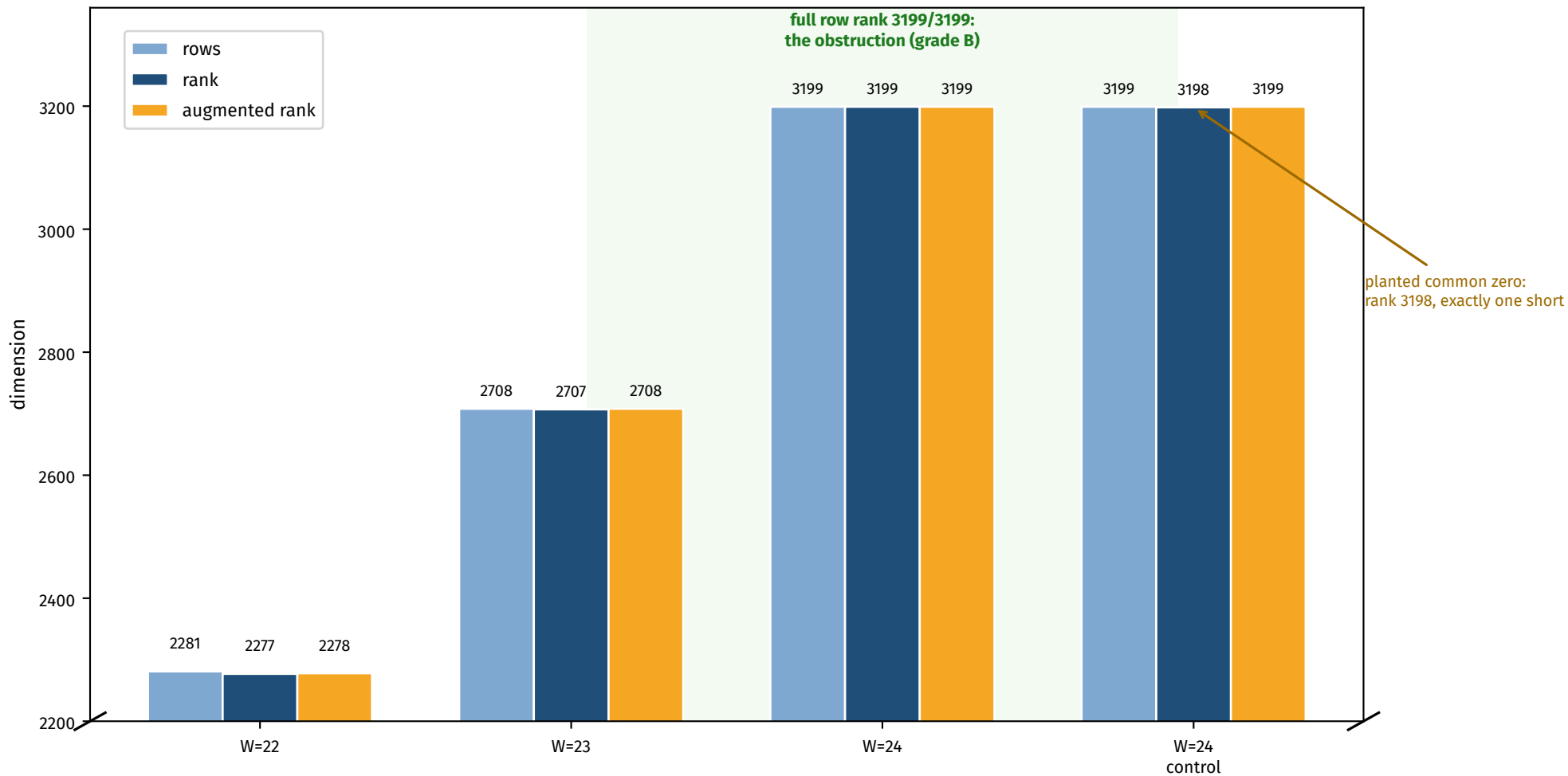
Macaulay rank profile at W = 22, 23, 24 ( p = 1000003 and p = 32003 ; identical)
