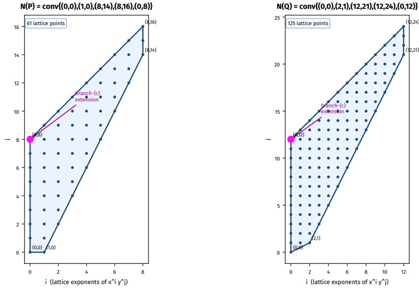
Figure 1: Branch-(c) Newton polygons, rendered from the exact vertex data of (1) (sourced at GGHV v1 lines 495 and 599–600). In each panel the branch-(a,b) sub-polygon is drawn in the lighter shade underneath; the extra branch-(c) vertices (0, 8) and (0, 12) are highlighted in the accent color. All lattice points are marked (61 for N(P) , 125 for N(Q) ); the ten vertex coefficients required nonzero by NewtonNfc are labelled. Rendered by figures/fig1_newton_polygons.py from the vertex lists.
