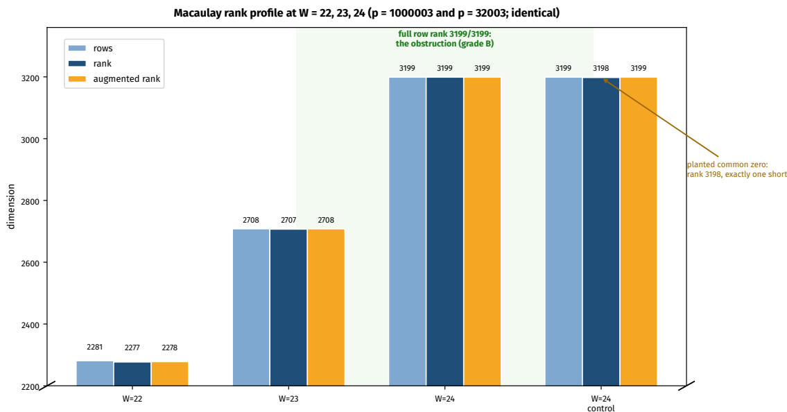
Figure 4: Macaulay rank profile at weights W = 22, 23, 24 , identical at both primes ( p = 1000003 and p = 32003 ). For each weight: bars for the number of rows (2281, 2708, 3199), the computed rank (2277, 2707, 3199), and the augmented rank, with the W = 24 group highlighted (full row rank 3199/3199, the obstruction). The fourth group shows the planted-common-zero control at W = 24 (rank 3198, exactly one short of full). Data source: step3b_rank_lift.log. Rendered by figures/fig4_ranks.py; the y -axis is truncated with a break mark to make the single-rank deficit visible.
