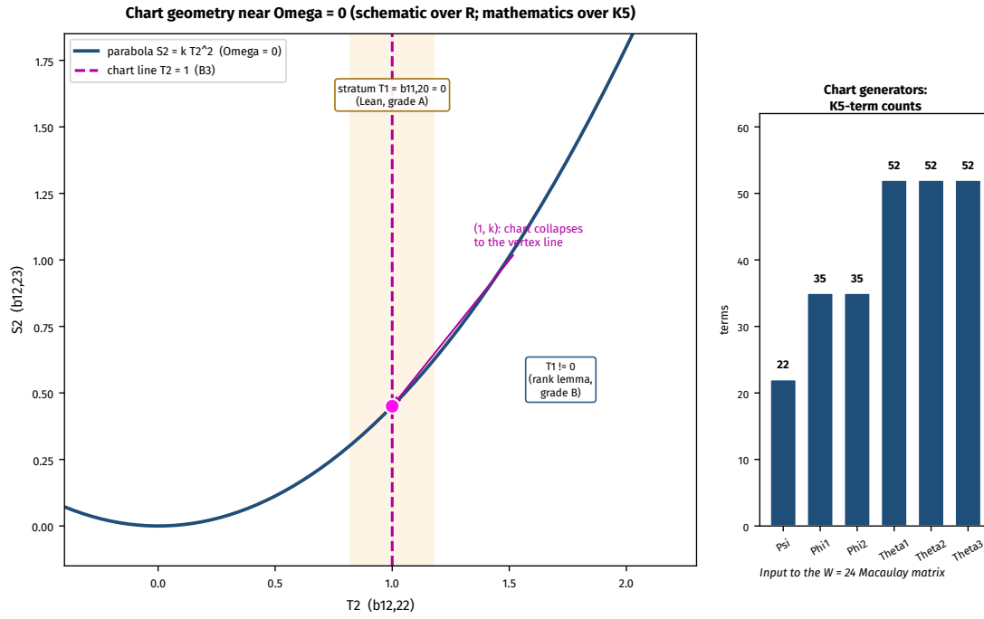
Figure 3: Chart geometry near \Omega = 0 . Main panel: the (T_2, S_2) -plane drawn schematically over \mathbb{R} for illustration (the mathematics is over K_5 ), showing the parabola S_2 = kT_2^2 from (6), the chart line T_2 = 1 (normalization B3), and their intersection (1, \kappa) ; the stratum T_1 = b_{11,20} = 0 is indicated as a transverse slice, with the T_1 = 0 stratum (Lean, grade A) and the T_1 \neq 0 stratum (rank lemma, grade B) labelled. Inset: the six chart generators' K_5 -term counts (22, 35, 35, 52, 52, 52), the input to the Macaulay matrix of §10. Rendered by figures/fig3_omega.py.
