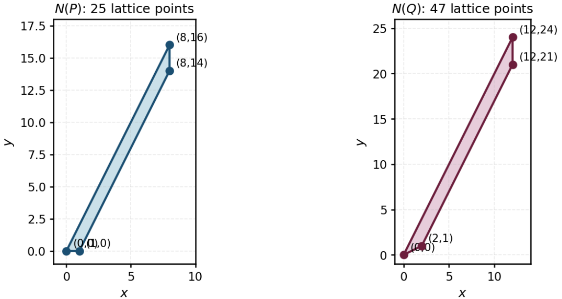
Figure 1: The branch (a,b) Newton polygons from [1, Proposition 4.3(2)], source-gated at v1 lines 495 and 599–600. N(P) has 25 lattice points; N(Q) has 47.
