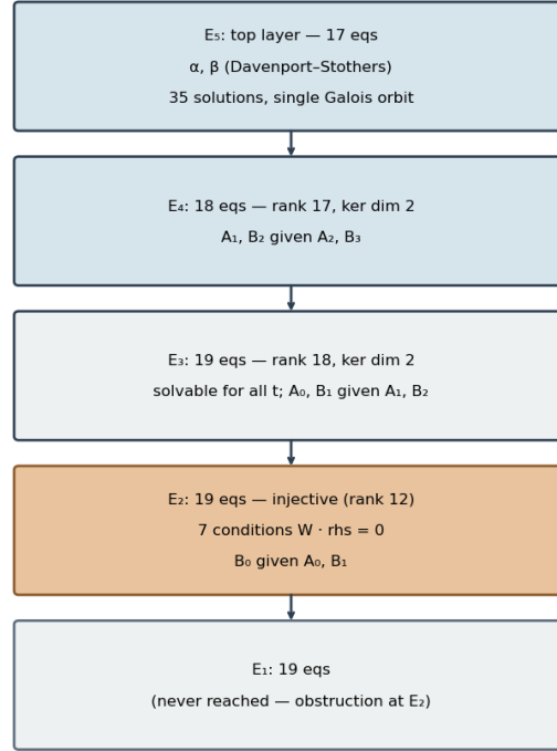
Figure 2: The triangular layer structure: 92 equations in five layers. Each layer is affine-linear in its unknowns given the solution above it.
