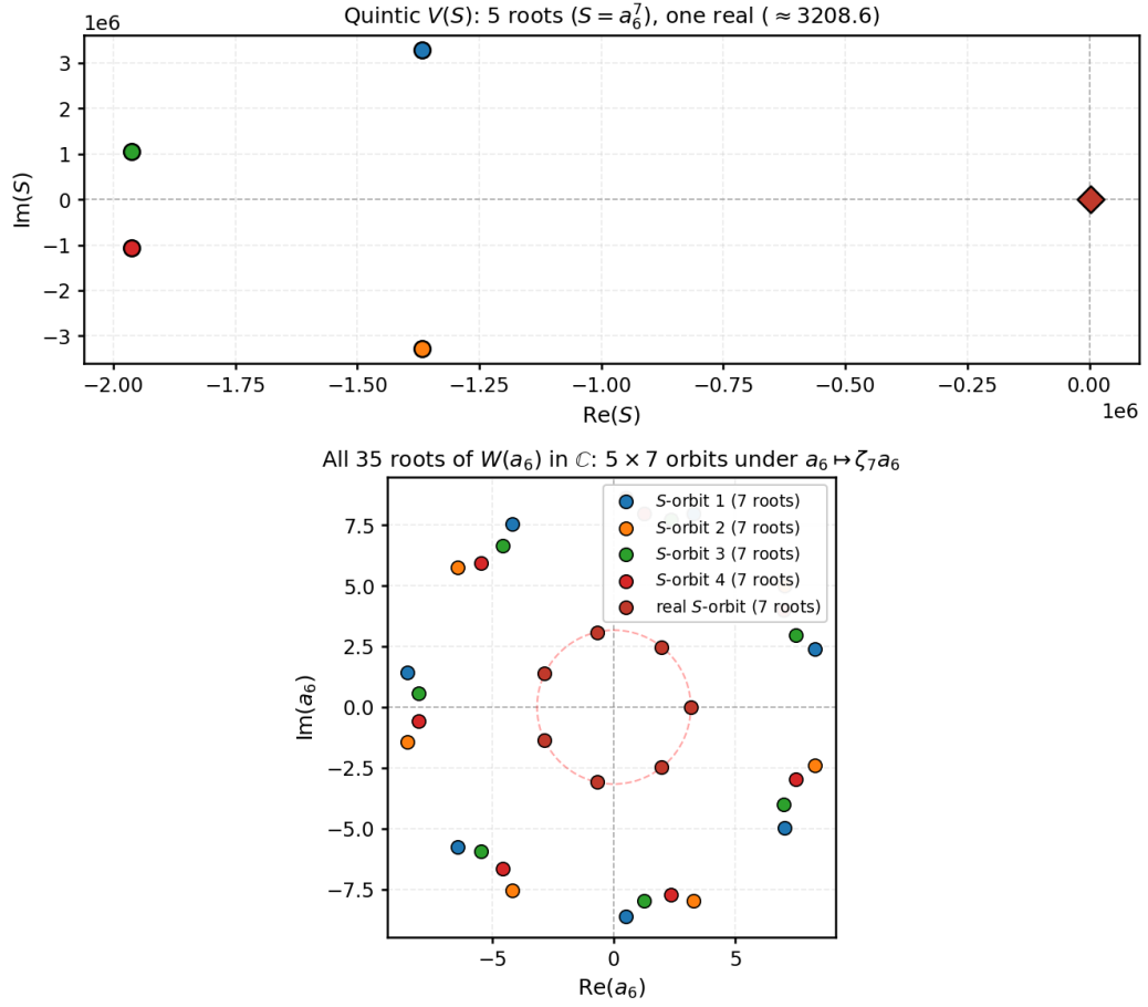
Figure 3: Top: the five roots of the quintic V(S) in the complex S -plane, computed from the integer coefficients; the real root S \approx 3208.61 is marked with a diamond. Bottom: all 35 roots of W(a_6) in \mathbb{C} , colored by S -orbit; each S \neq 0 lifts to 7 values of a_6 via 7th roots of unity. The dashed circle marks the real S -orbit. The 35 roots form a single Galois orbit over \mathbb{Q} .
