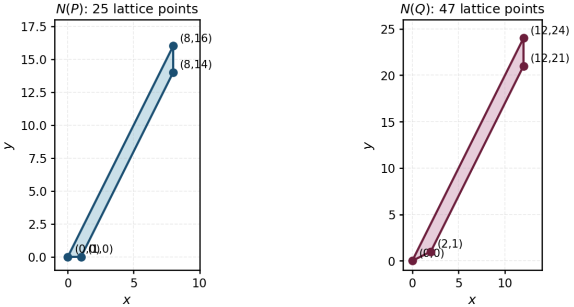
Figure 1: The branch (a,b) Newton polygons from [1, Proposition 4.3(2)], source-gated at v1 lines 495 and 599–600. N(P) has 25 lattice points; N(Q) has 47.
