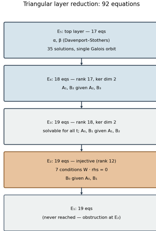
Figure 2: The triangular layer structure: 92 equations in five layers. Each layer is affine-linear in its unknowns given the solution above it.
