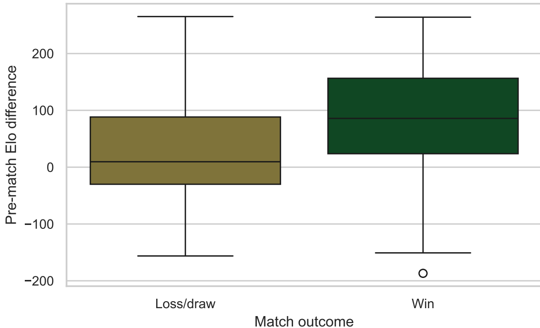
Pre-match Elo difference by match outcome
