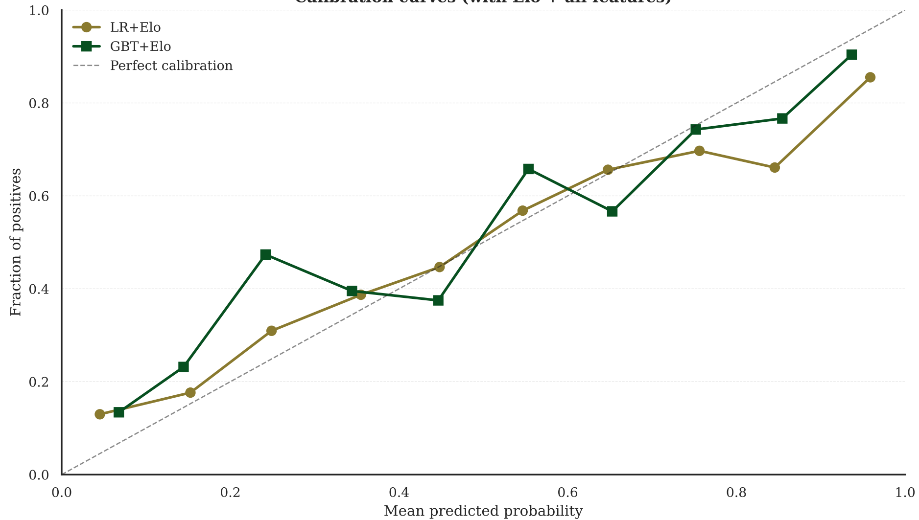
Calibration curves (with Elo + all features)
