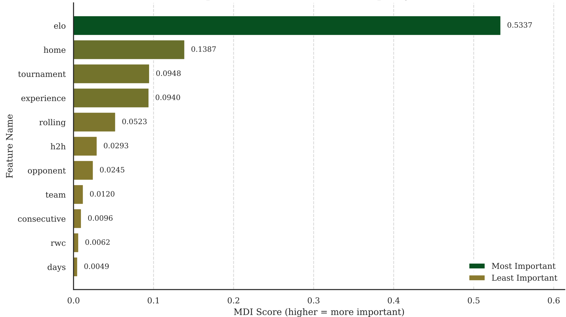
Feature Importance (Mean Decrease in Impurity) – GBT Model
