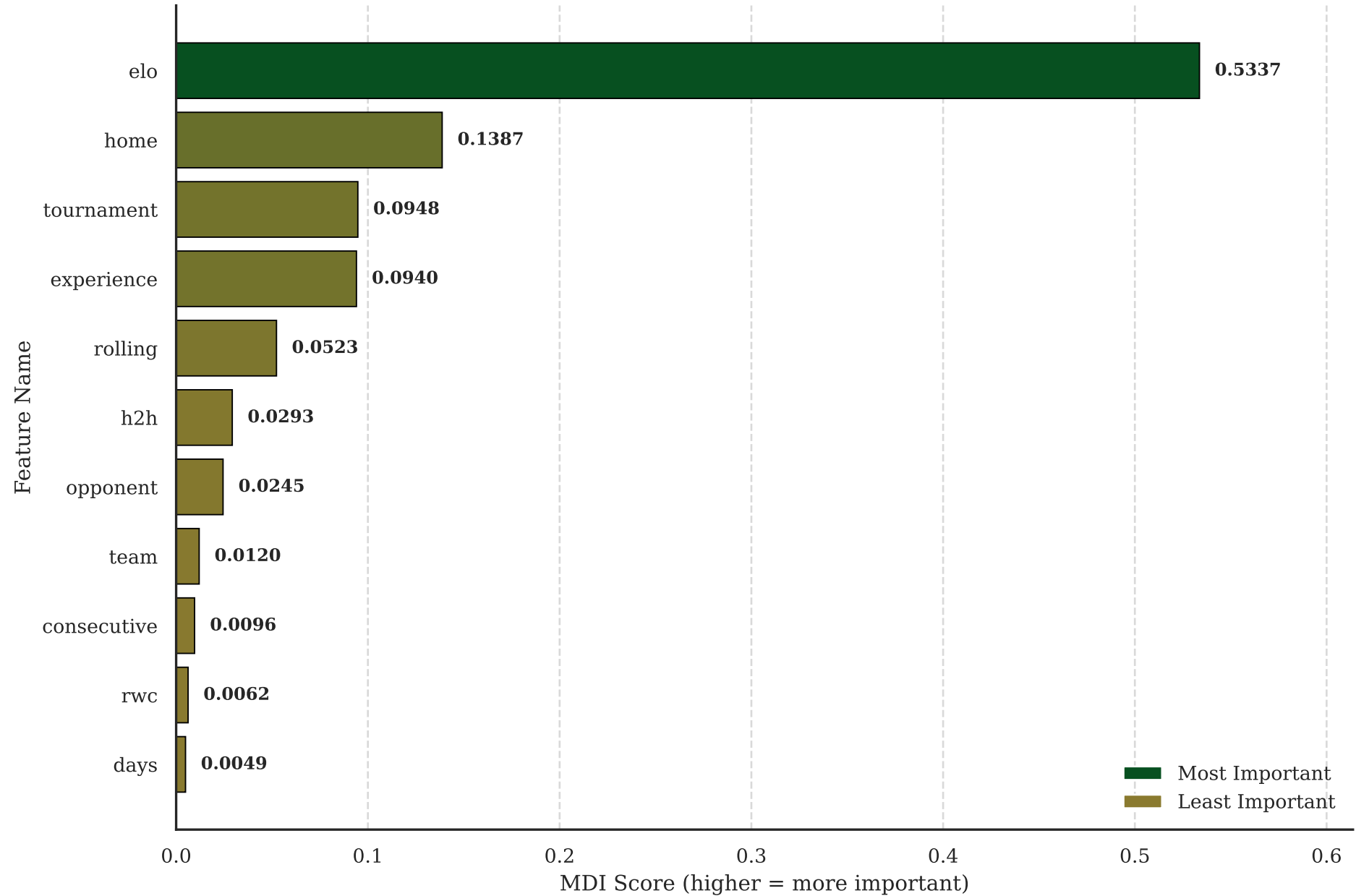
Feature Importance (Mean Decrease in Impurity) — GBT Model
