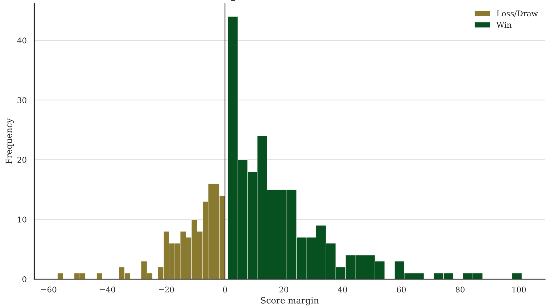
Score margin distribution — South Africa
