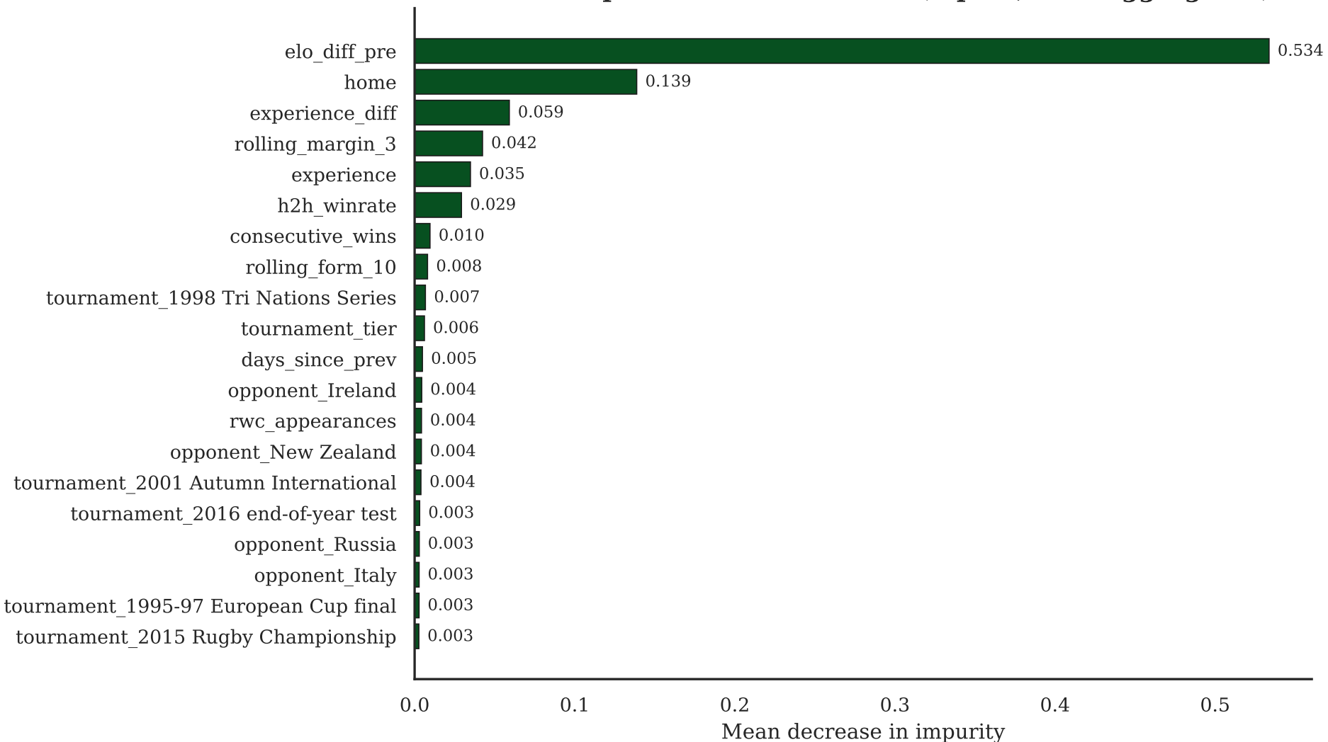
Feature importance — GBT + Elo (top 20, OHE aggregated)
