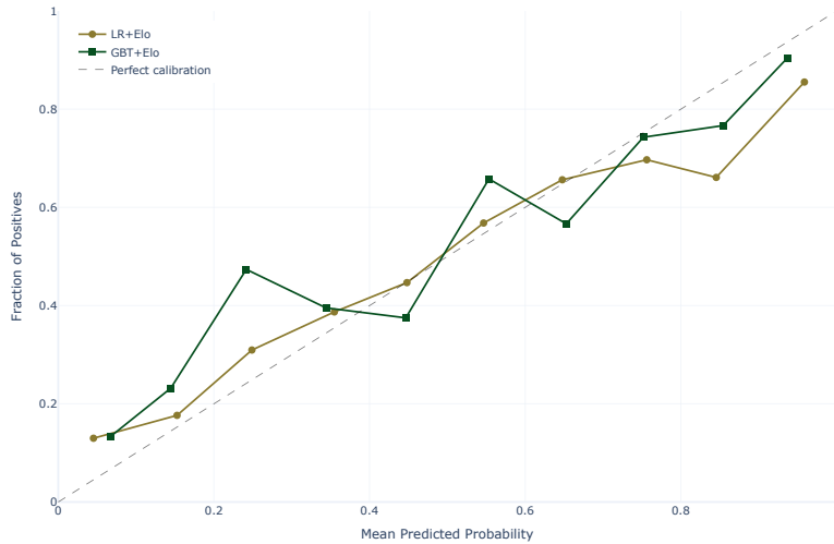
Figure 6: Calibration curve (GBT+Elo) showing predicted vs. observed win probabilities. Points near the diagonal indicate good calibration. The dashed line represents perfect calibration.
