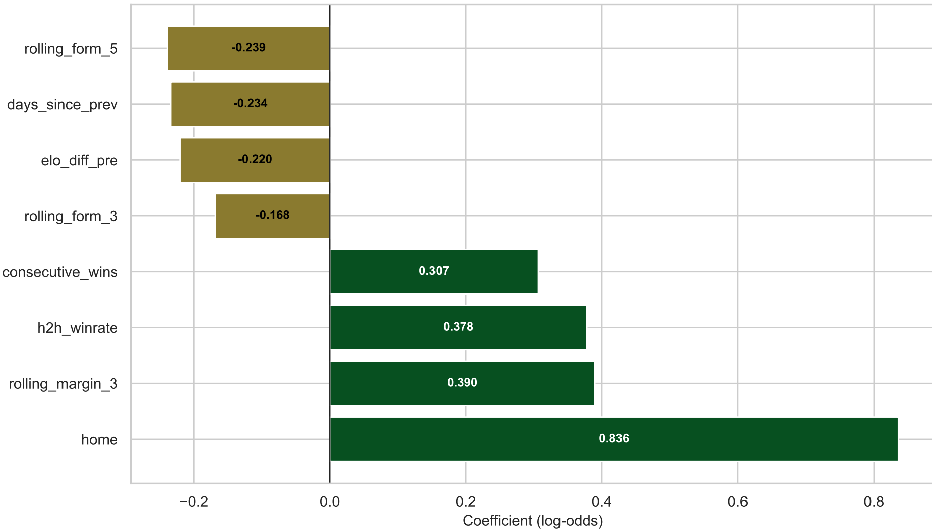
Feature Importance – Logistic Regression (Elo Model)
