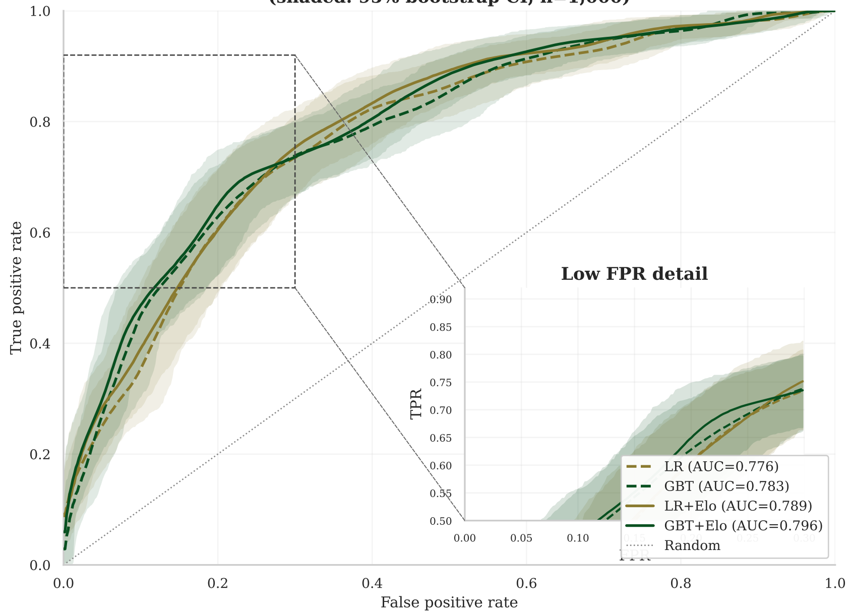
ROC curves: impact of Elo feature (shaded: 95% bootstrap CI, n=1,000)
