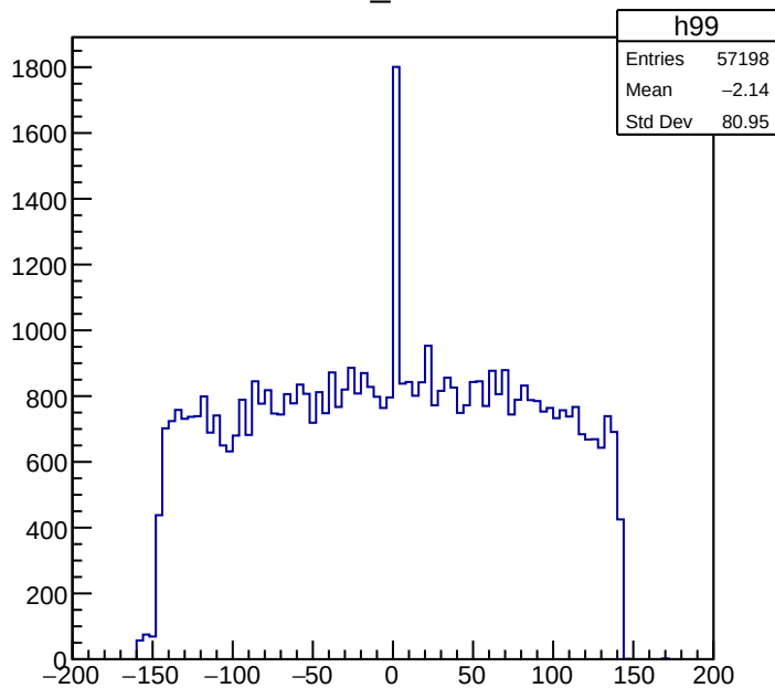
Z_vtx
