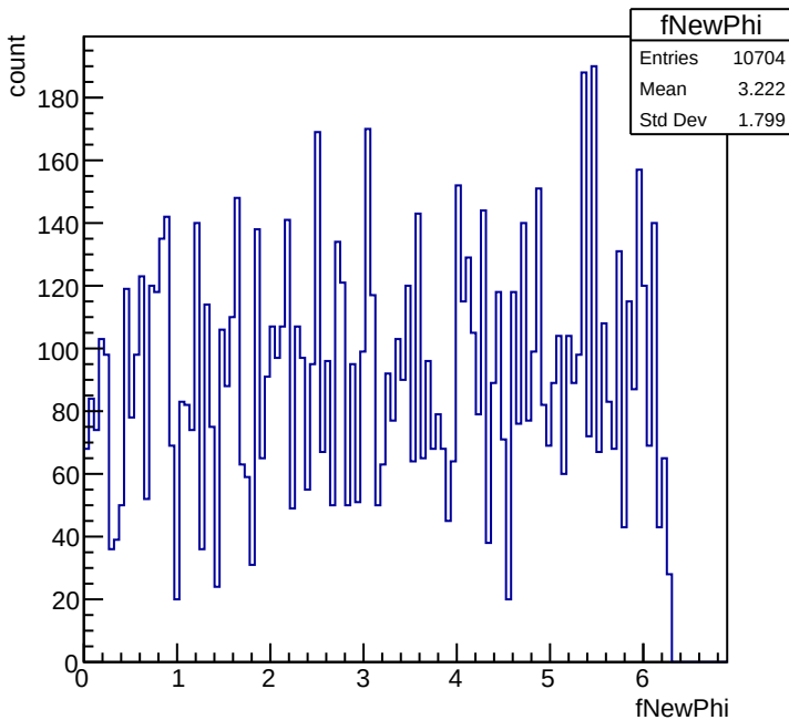
fNewPhi
