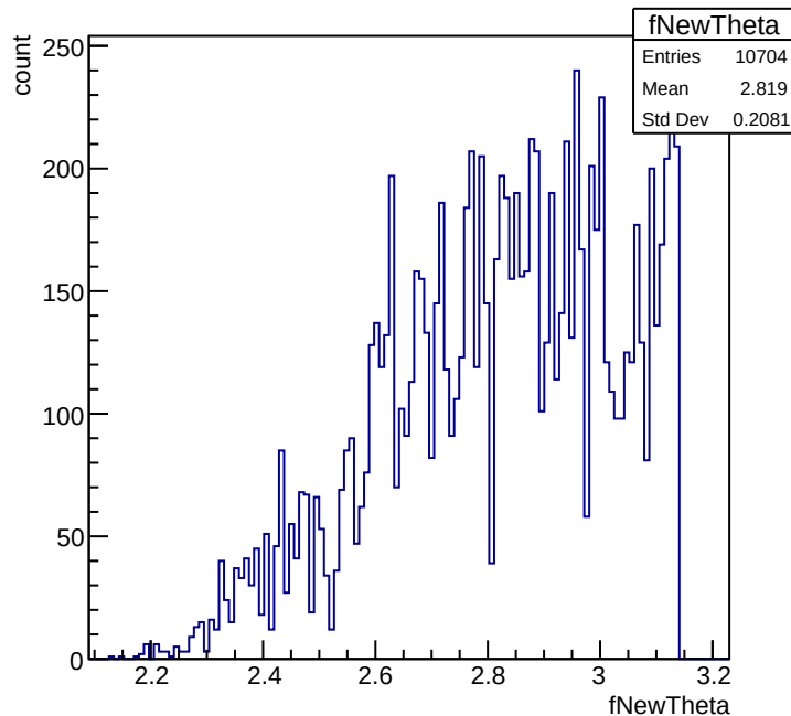
fNewTheta
