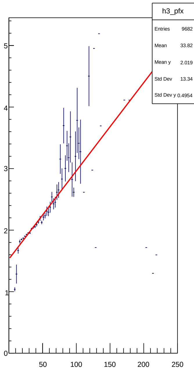
Finger Edep vs Nphot
