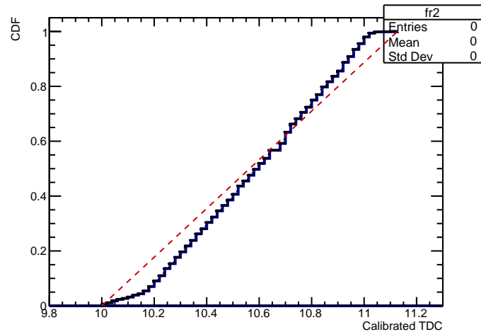
Calibrated CDF vs ideal
