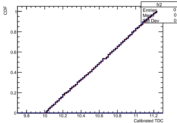
Calibrated CDF vs ideal
