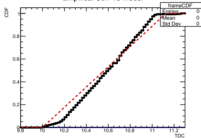
Empirical CDF vs model
