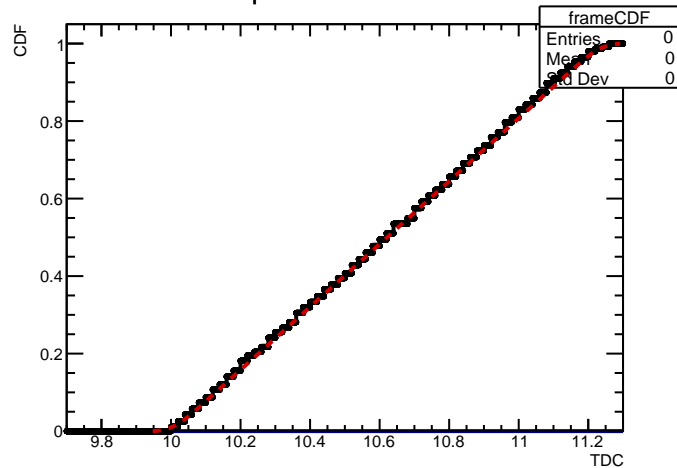
Empirical CDF vs model
