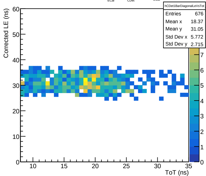
Bar 1L30 diagonal component ( 1 < t_{\text{ECal}} < 18 , |-27 - 0.73 t_{\text{ECal}}| < 3 ns)
