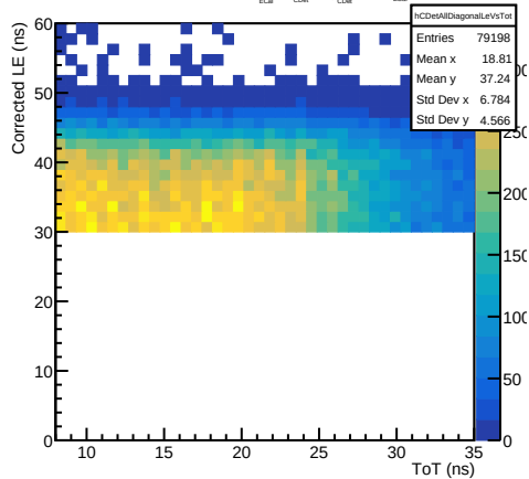
All CDet bars: diagonal component ( t_{\text{ECal}} > 1 , t_{\text{CDet}} > 30 , |t_{\text{CDet}} - 27 - 0.73t_{\text{ECal}}| < 3 ns)
