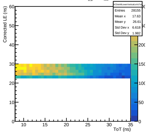
All CDet bars: lower vertical component ( -5 < t_{\text{ECal}} < 1 , 23 < t_{\text{CDet}} < 30 ns)
