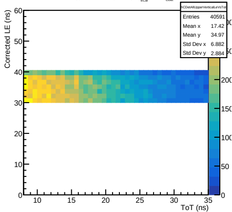
All CDet bars: upper vertical component ( -5 < t_{\text{ECal}} < 1 , 30 < t_{\text{CDet}} < 40 ns)
