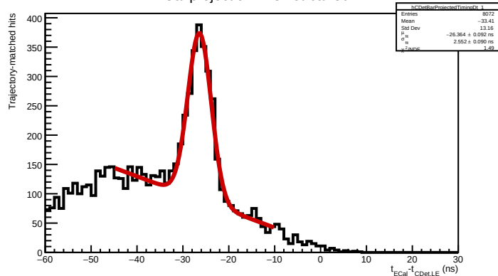
ECal projection in CDet bar 30
