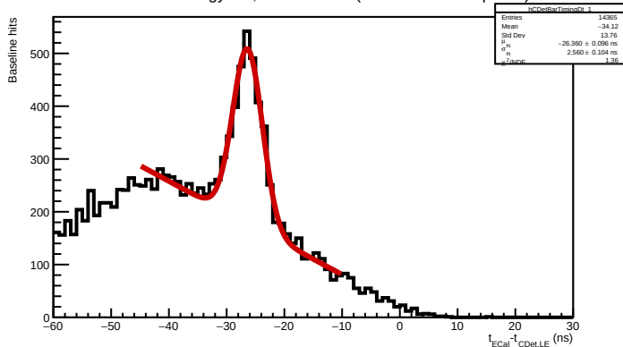
After ECal energy cut, CDet bar 30 (all instrumented pixels)
