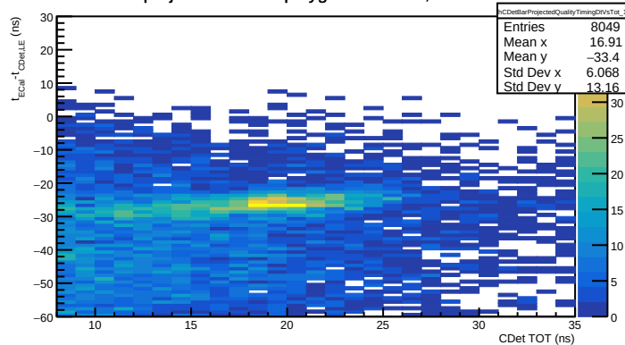
ECal projection + TOT/polygon selection, CDet bar 30
