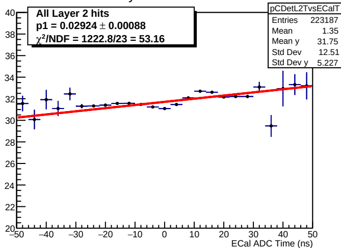
CDet Layer 2 t vs ECal Time
