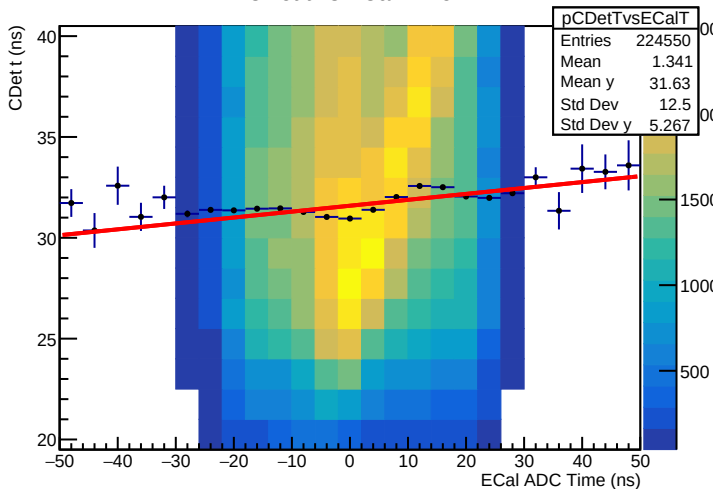
CDet t vs ECal Time
