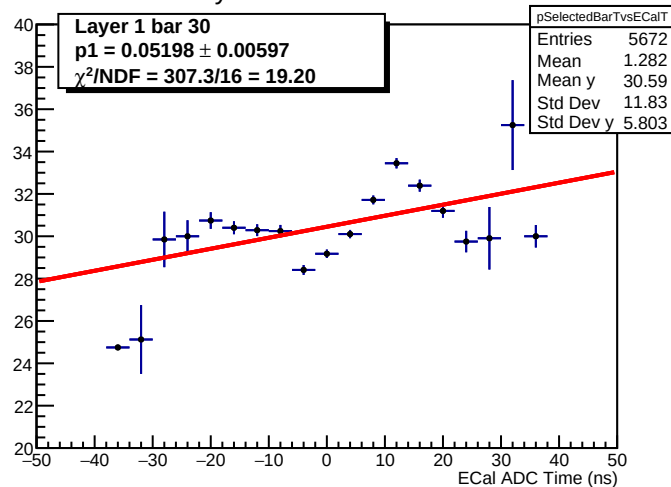
CDet Layer 1 bar 30 t vs ECal Time
