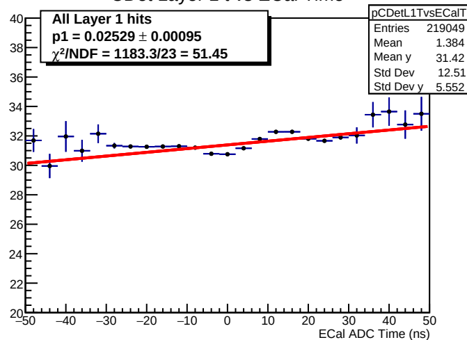
CDet Layer 1 t vs ECal Time
