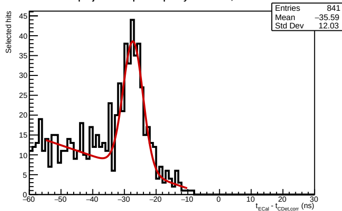
ECal projection + pulse-quality selection, CDet bar 30
