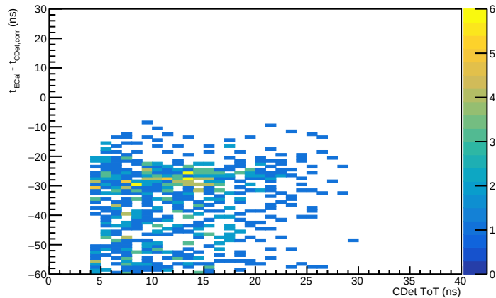
ECal projection + pulse-quality selection, CDet bar 30
