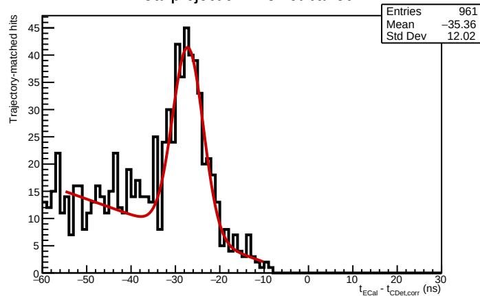
ECal projection in CDet bar 30
