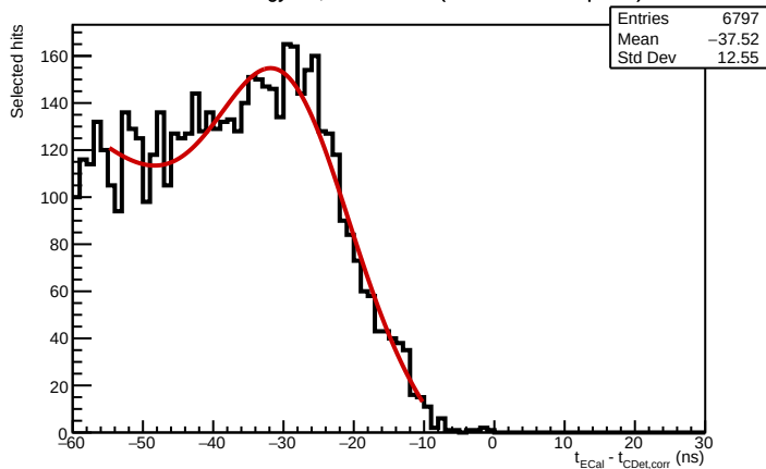
After ECal energy cut, CDet bar 30 (all instrumented pixels)
