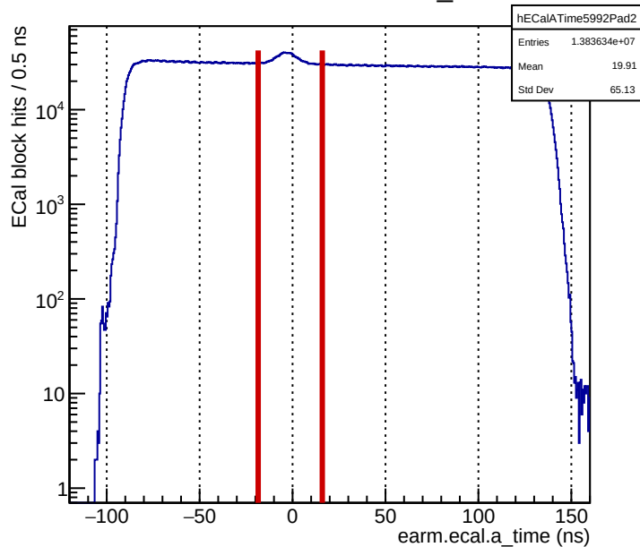
Run 5992: earm.ecal.a_time
