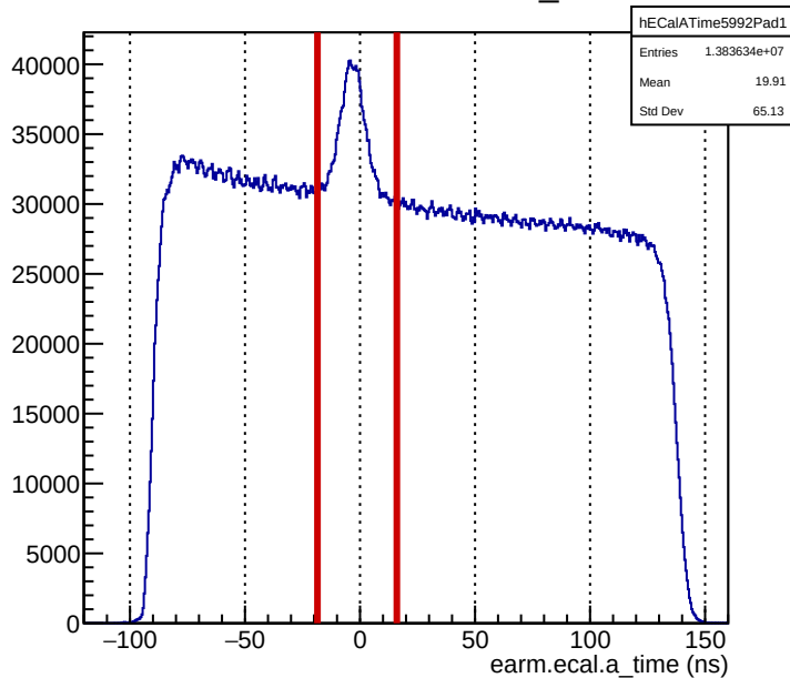
Run 5992: earm.ecal.a_time
