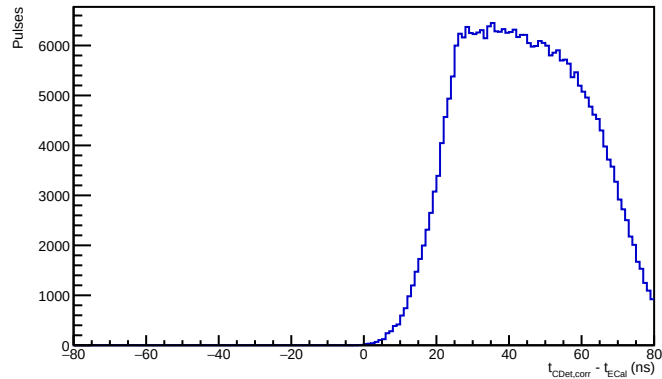
Layer comparison
