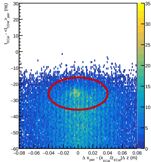
Accepted pairs
