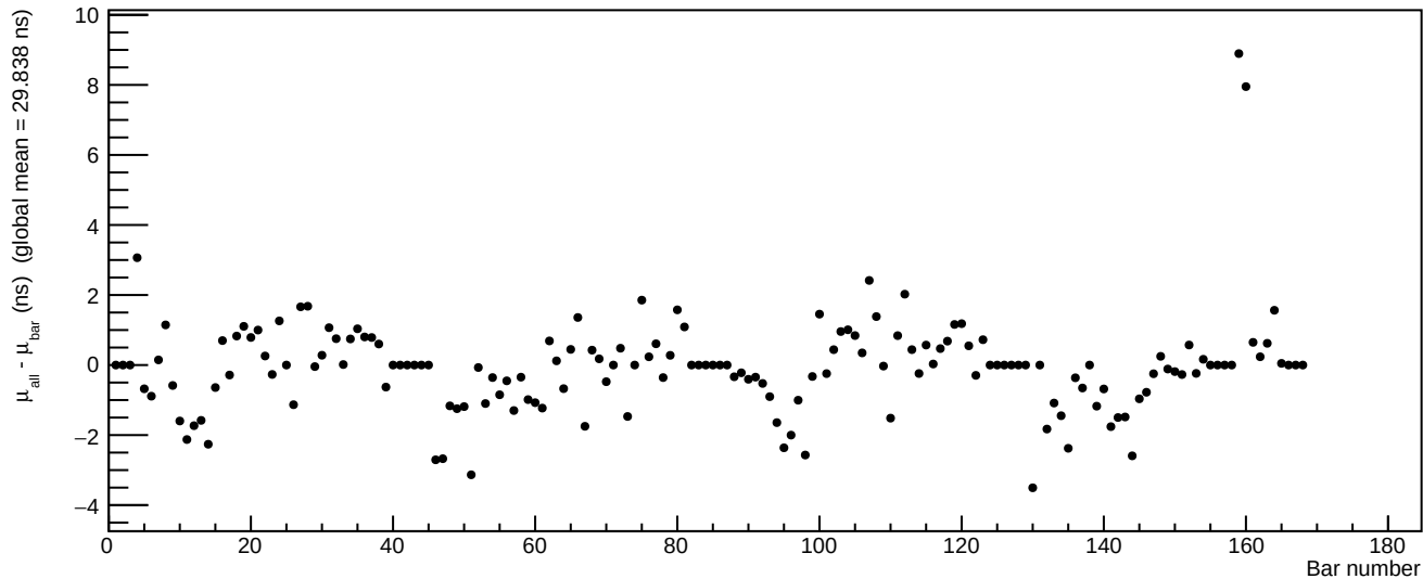
Residual LE offsets vs Bar
