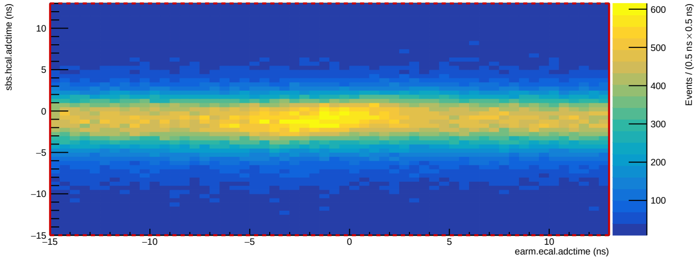
Run 6077: HCal vs. ECal ADC time
